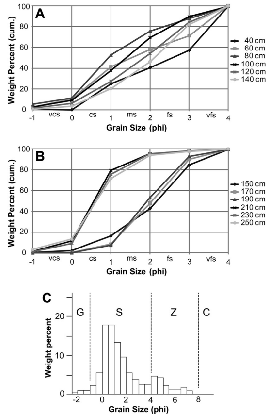
Figure 12. Cumulative grainsize distributions for samples sieved a 1- \phi intervals. Unanalyzed pan fraction (finer than 3 \phi ) arbitrarily plotted at 4 \phi . Some clasts coarser than -1 \phi omitted. Sample numbers are depth (centimeters) of sample below surface. Letter code on abscissa are Wentworth designation of sand sizes: vc = very coarse, c = coarse, m = medium, f = fine, vf = very fine. Recalculated from data supplied by R.M. Gramly. A. Top of flood bar (140–80 cm depth) and overlying eolian deposit (60–40 cm depth). B. Flood bar: coarser layer (250–210 cm depth) and overlying finer layer (190–150 cm depth). C. Grainsize histogram redrawn from the detailed sieving in Mehringer (1989b). From his sediment column II, sample 3 is 65 cm below surface and 12 cm below artifact layer. Gravel, sand, silt, and clay fields indicated. Example selected from 65 histograms.
