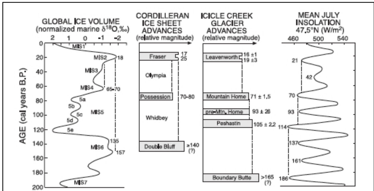
Fig. 15. Chronology and relative extent of Icicle Creek glacier advances compared with those of the Puget Lobe of the Cordilleran Ice Sheet. These records are compared with the curve of global ice volume, based on the standard marine oxygen-isotope record (Martinson and others, 1987), and with a curve of summer (July) insolation for the latitude of the Icicle Creek glacier (47.5° N; data from M. F. Loutre, personal communication, 2001). Whereas the relative magnitude of the ice sheet advances approximately match those of the last three glacial marine-isotope stages (MIS 2, 4, and 6), the relative magnitudes of the Icicle Creek glacier advances match those of prominent insolation minima (21,000, 70,000, 92,000, and 114,000 years ago) of the last 160,000 years.
